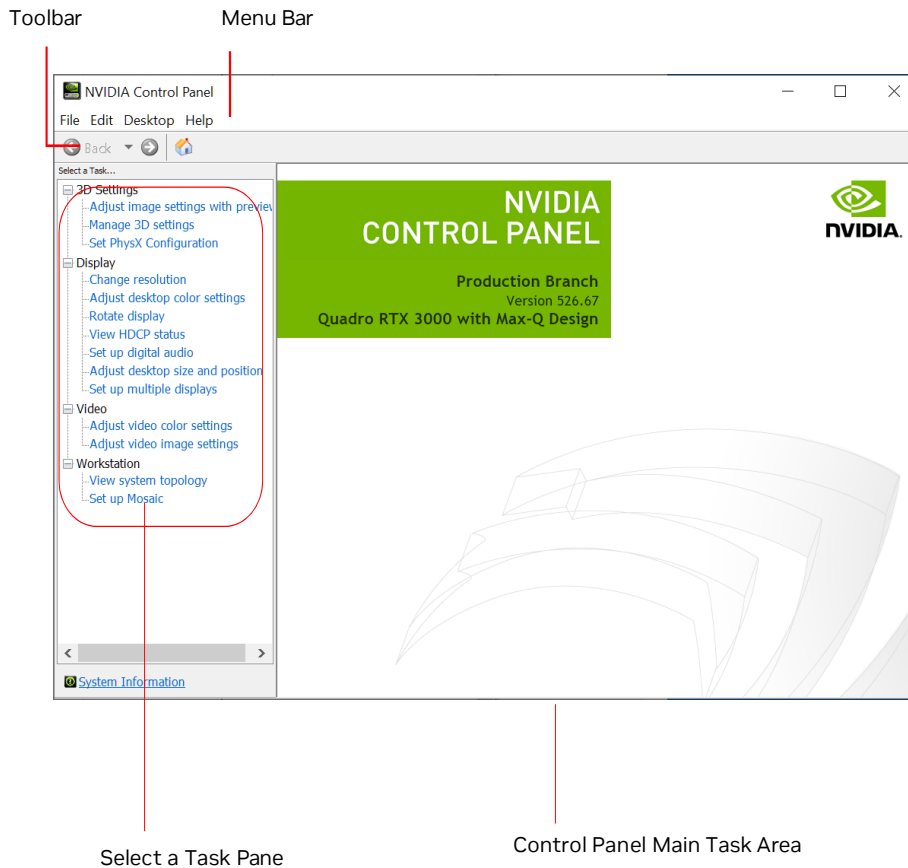
Figure 1. NVIDIA Control Panel
