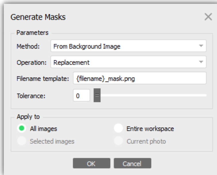
"Generate Masks" dialog
