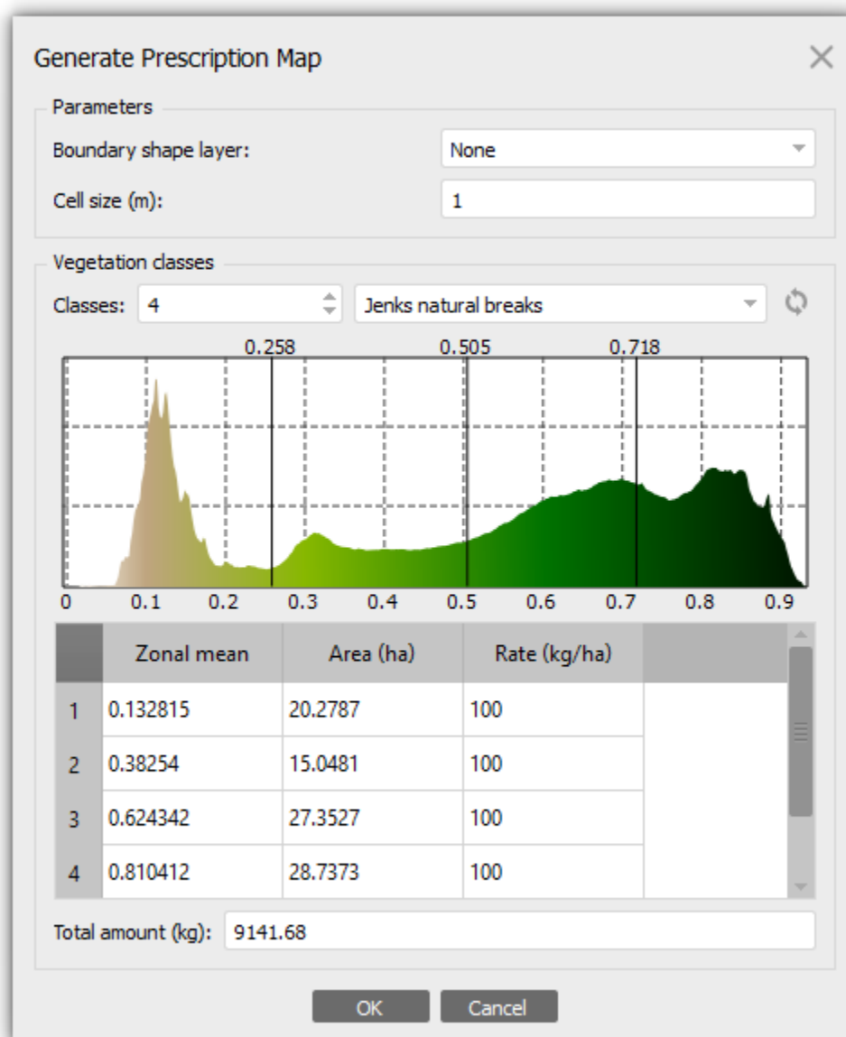
"Generate Prescription Map" dialog window
