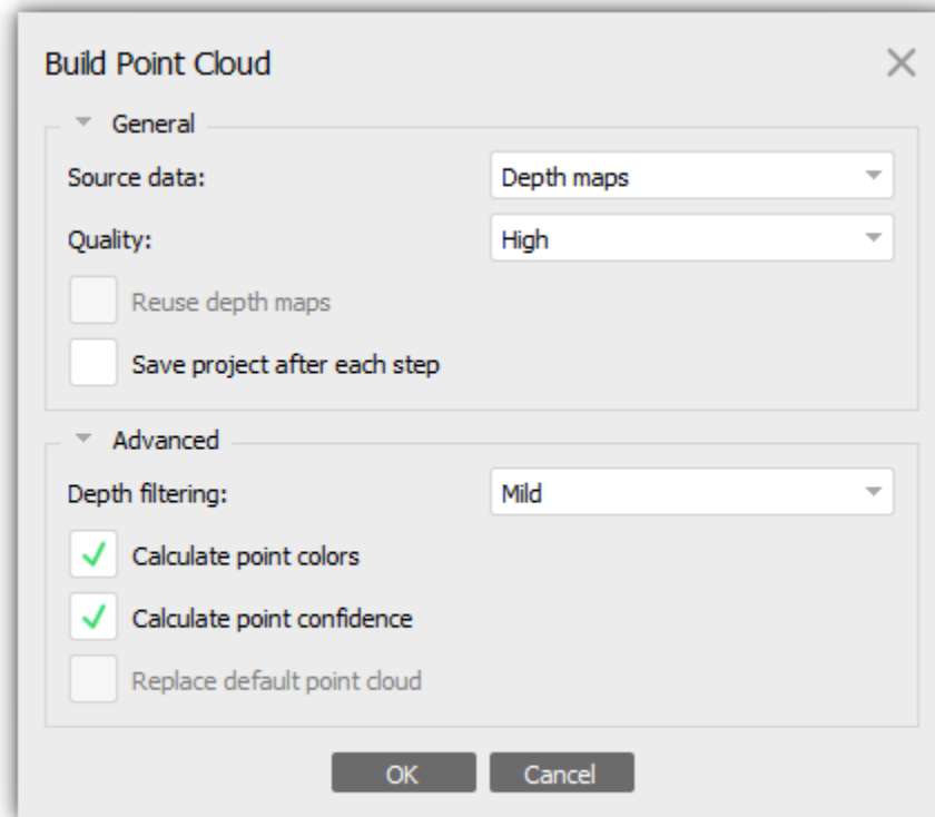
"Build Point Cloud" dialog
